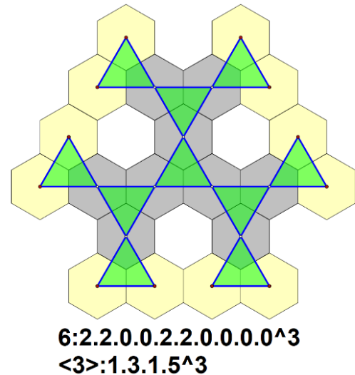
Figure 29: A polygon represented in both equilateral and equiangular polytile notation
