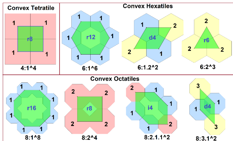
Figure 4: One tetratile, three hexatiles and four octatiles
