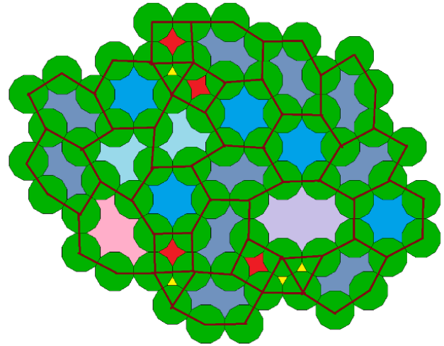
Figure 2: Convex equilateral polygons (outlined) from edge-to-edge dodecagons
