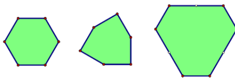
Figure 1: Regular hexagon, isotoxal (equilateral), and isogonal (equiangular)
