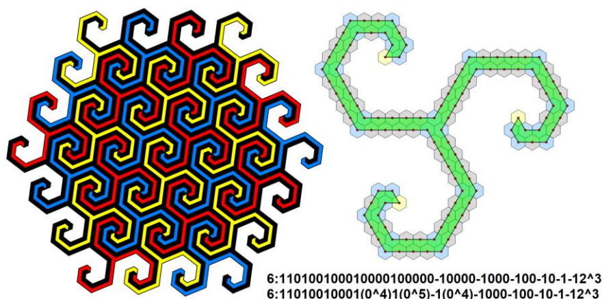
Figure 12: A monohedral hexatiles tri-spiral
