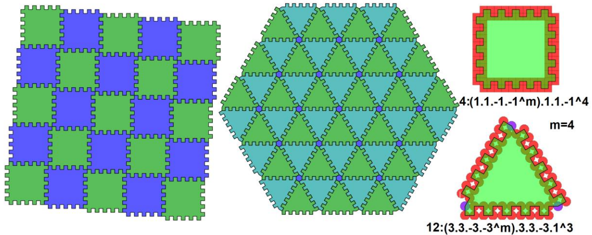
Figure 25: Tilings made with polytiles extended by square waves
