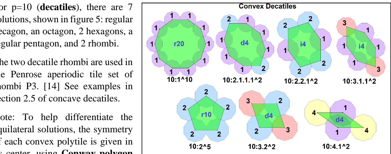
Figure 5: Set of convex decatiles
